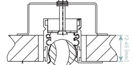
Installation to a baffle by means of visible screws
